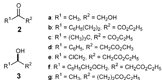
Figure 3. Ketone substrates 2 and hydrogenation products 3 .
