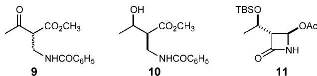
Figure 4. Structures of compounds 9 , 10 , and 11 .
