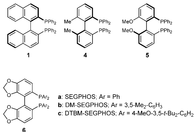
Figure 2. Structures of ligands 1, 4, 5, and 6.
