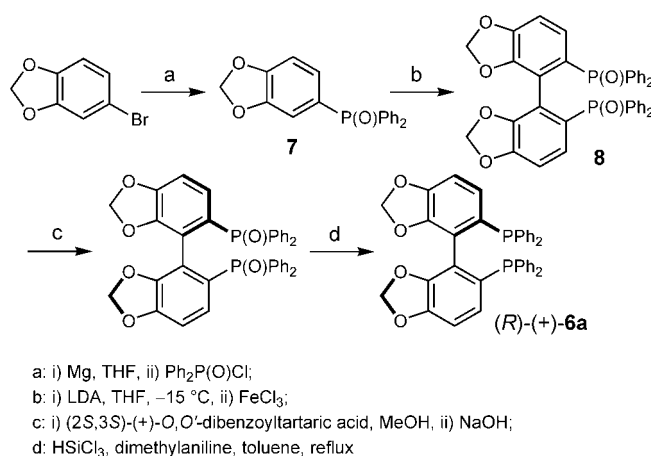
Scheme 1. Synthesis of the ( R )-(+)-SEGPHOS ligand.
