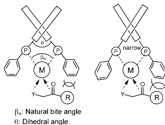
Figure 1. Steric considerations based on the effect of varying the dihedral angle ( \theta ) in biaryl backbone.
